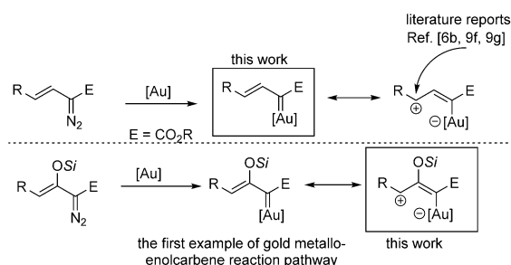
Scheme 2. Known reaction pathway and novel reaction modes (our work).
