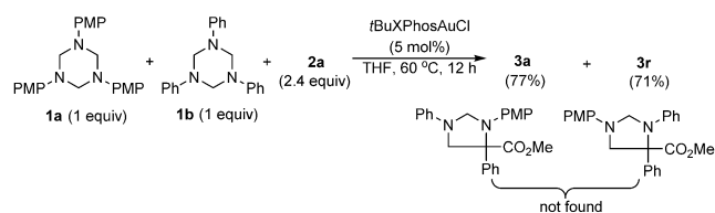
Scheme 4. Control experiments.
