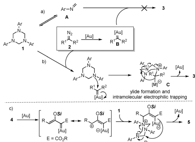
Scheme 5. Proposed mechanisms.
