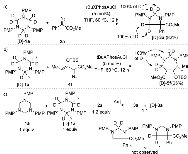
Scheme 3. Deuterium-labeling experiments. THF = tetrahydrofuran.
