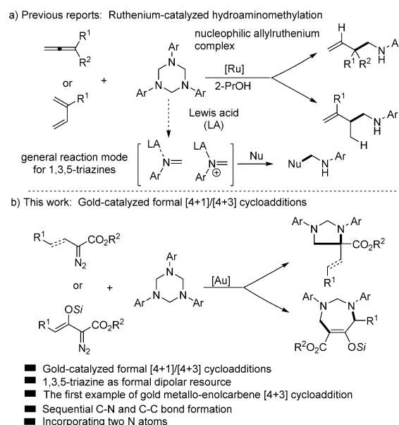
Scheme 1. Previous reports and our approach. LA = Lewis acid, Si = silyl protecting group.
